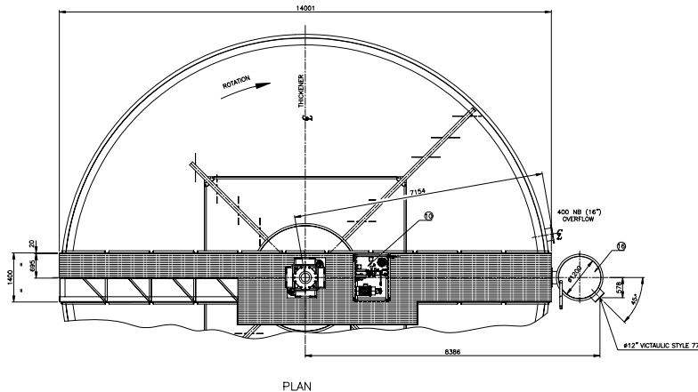
Center Support
