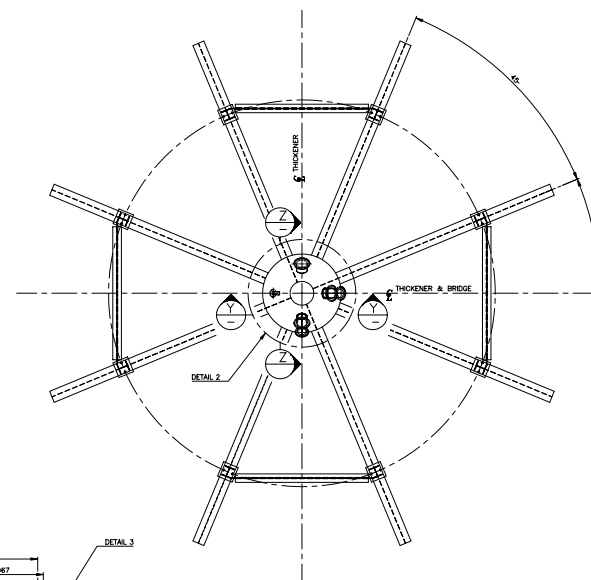
PLAN ON SUPPORT BEAM
