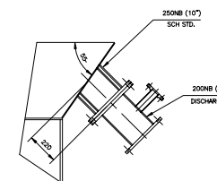
DETAIL 3
